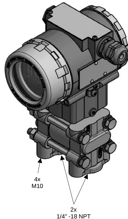
code N31 1/4" - 18 NPT vertical / fixing M10
