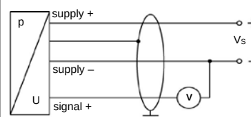
3-wire-system (voltage)
